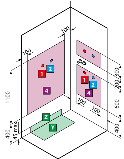
Version Links Version Rechts per modelli A 90x70 - A 100x70 - A 100x80 - 2P 120x80
