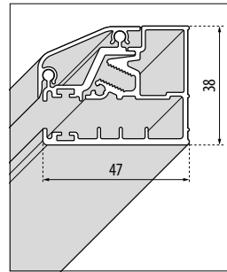
WALL side panel
